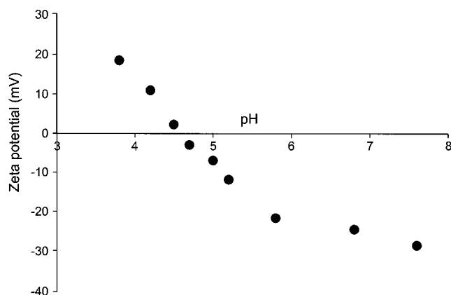
Fig. 1. Influence of the solution pH on the zeta potential (BSA concentration: 1.0 wt% in 10 mM KCl).
